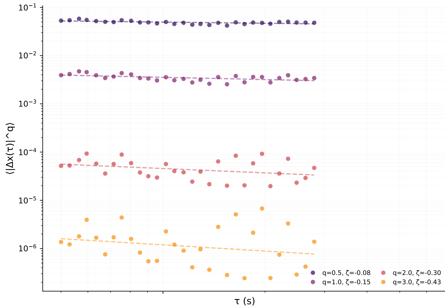
S-wave
