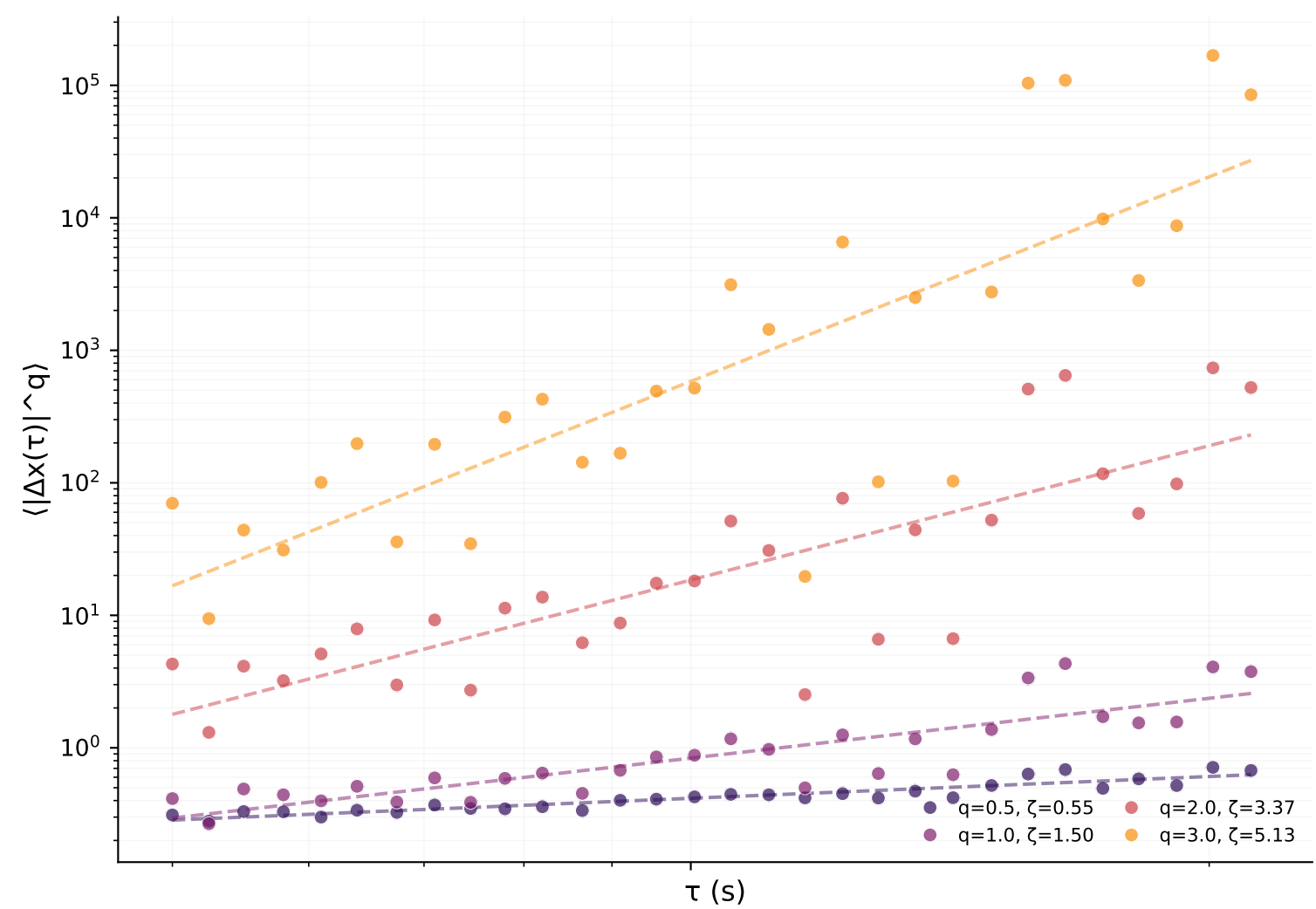
Coda
